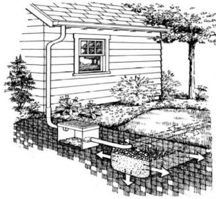
Dry Well (seepage pit)
