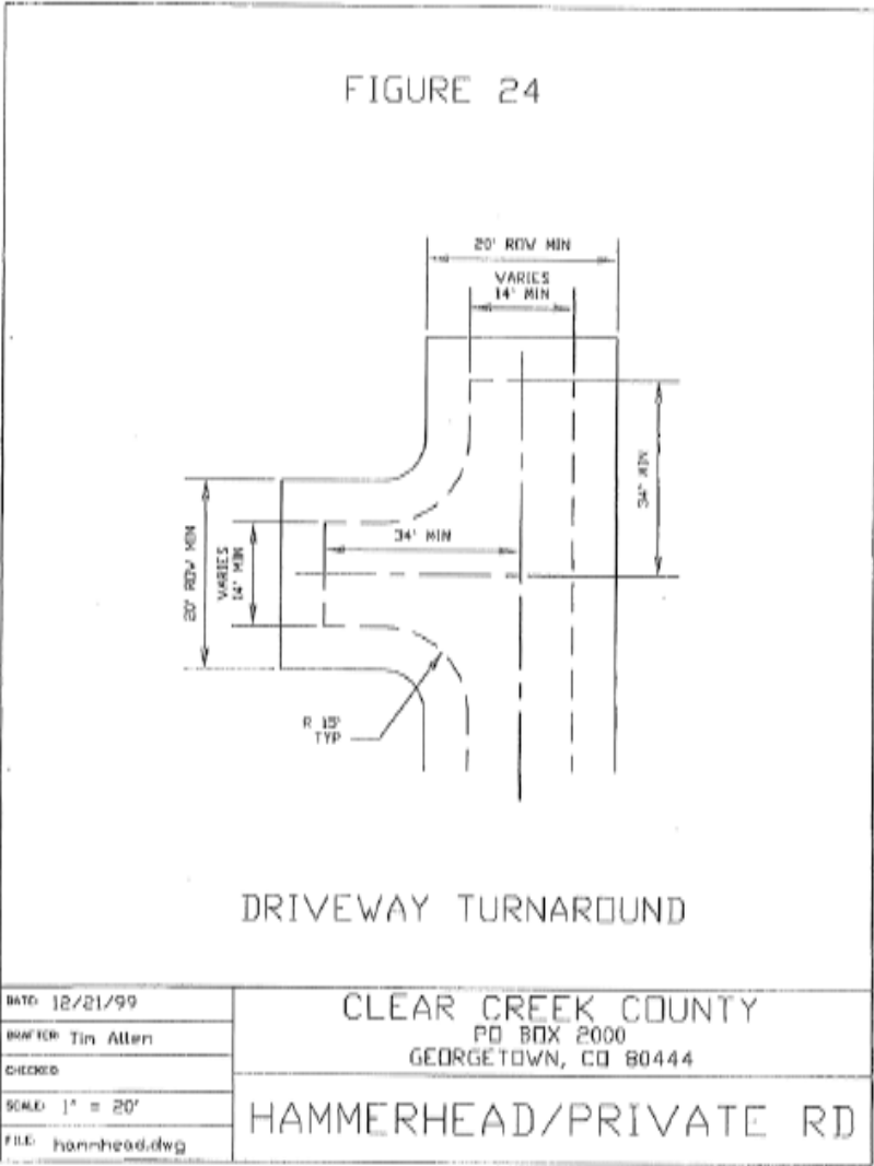
Figure 24 – Driveway Turnaround
