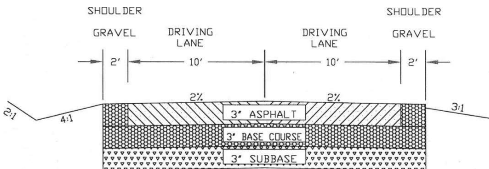
Typical Cross Section for a Primitive Status Road
