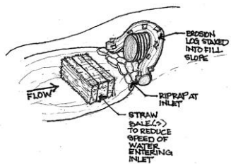
Temporary Inlet Protection
