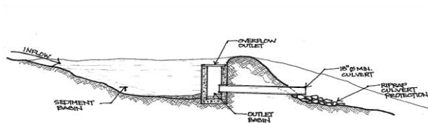
Sediment Basin Section BMP: CONSTRUCTION FENCE
