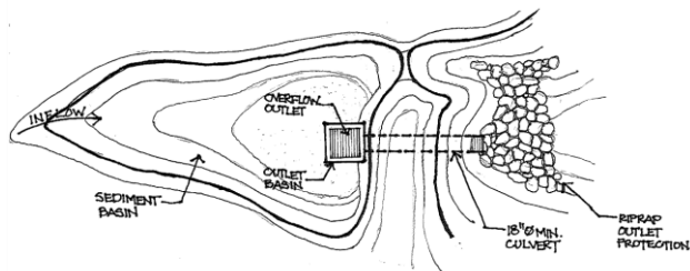
Sediment Basin
